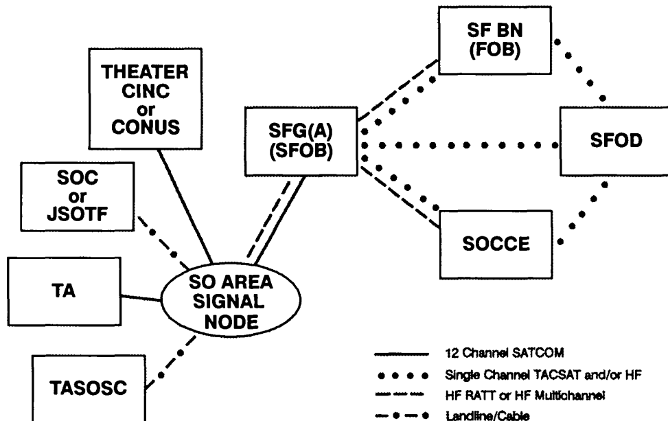
Figure 5-22. Type SF Communications in an Undeveloped Theater.
