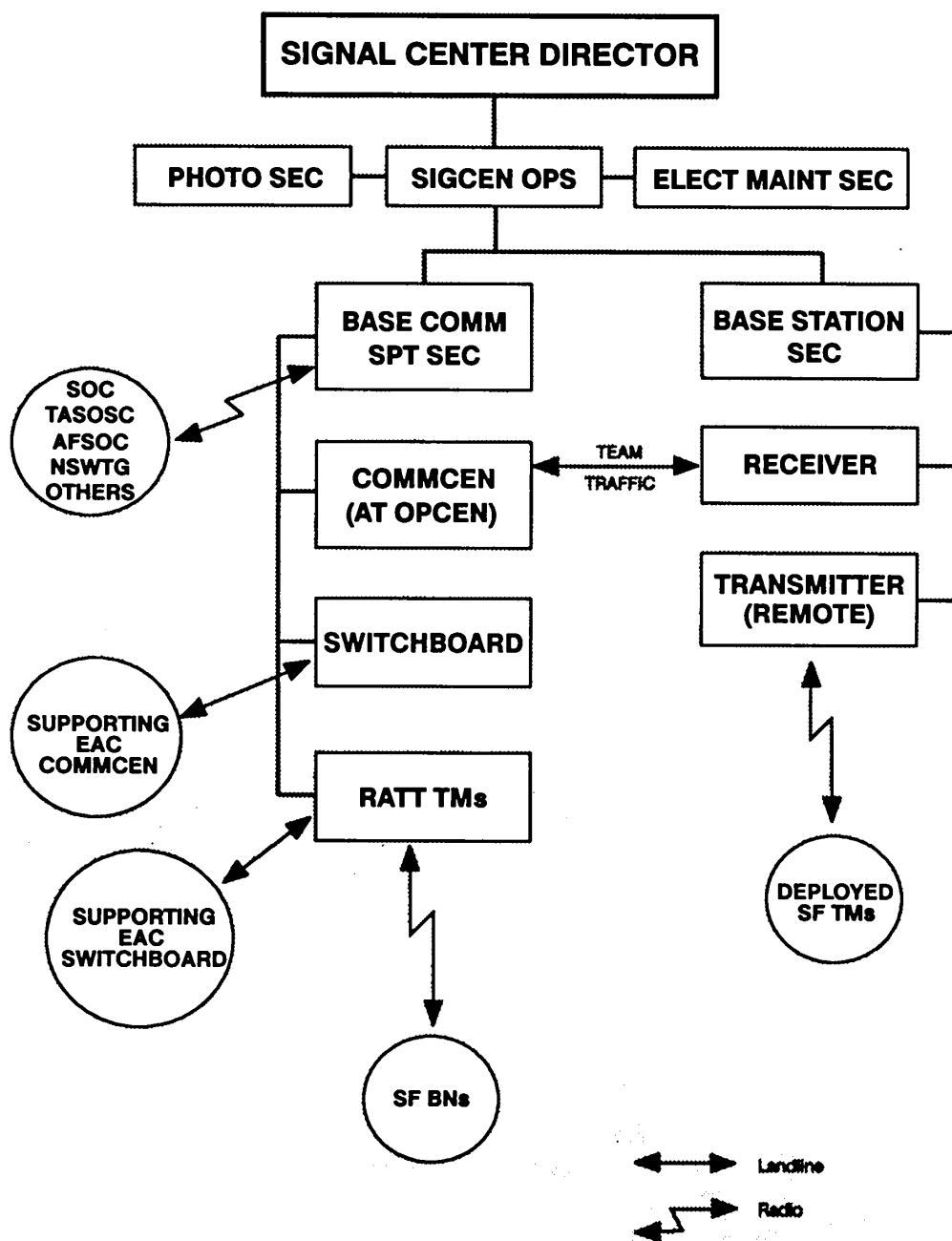
Figure 6-6. A Type SF Signal Center.
